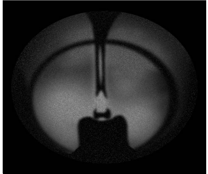
Figure 231: Burning in Supercritical Water. You are looking through a thick, sapphire window at combustion in supercritical water (SCW) at 450°C (842°F) and 1,000 bars (14,500 psi). The tube at 6 o'clock is injecting oxygen into the SCW at 3 mm 3 /sec. Oxygen unites with methane (CH 4 ) that is dissolved in the SCW and releases heat which, in turn, releases more oxygen in the water (H 2 O → H + OH → 2H + O). The resulting spontaneous combustion produces CO 2 and excess heat as long as fuel (in this case, carbon) is available. 9
