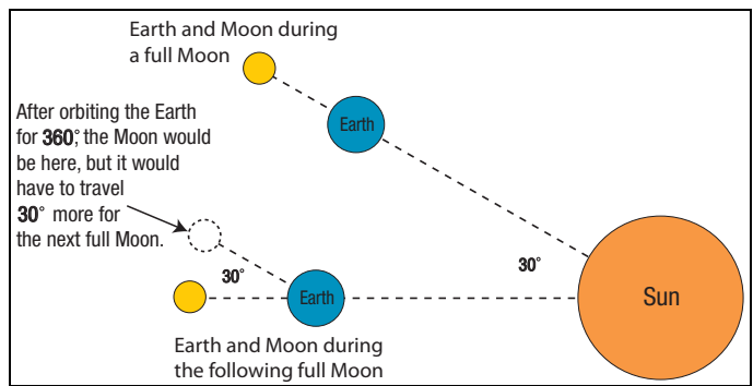
Figure 227: Synodic Period, the Time from Full Moon to Full Moon. Before the flood, a lunar month (or moonth) was 30 days, so the Moon had to revolve around the Earth 30° more than one complete revolution—or 390° total.
