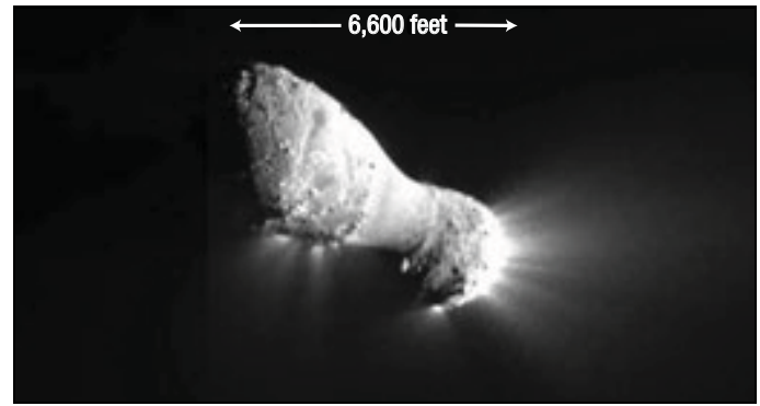
Figure 155: Comet Hartley 2. On 4 November 2010, the Deep Impact spacecraft passed within 435 miles of Comet Hartley 2 and took this photograph. Hartley 2 has a peanut shape, as does asteroid Itokawa (shown in Figure 154) and some other asteroids and comet nuclei, because they all formed by the same special mechanism.
