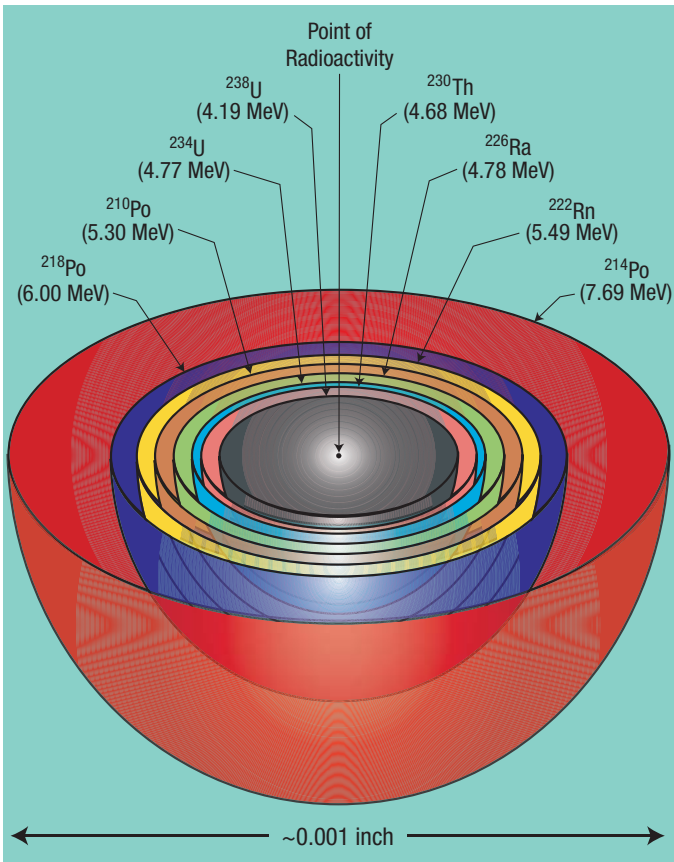
Figure 171: Radiohalos from the ^{238}\text{U} Decay Series. Suppose many ^{238}\text{U} atoms were concentrated at the point of radioactivity shown here. Each ^{238}\text{U} atom eventually ejects one alpha particle in a random direction, but at the specific velocity corresponding to 4.19 million electron volts (MeV) of energy—the binding energy released when ^{238}\text{U} decays. That energy determines the distance traveled, so each alpha particle from ^{238}\text{U} ends up at the gray spherical shell shown above. (Alpha particles from daughter isotopes will travel to different shells.) Each sharply defined halo requires the ejection of about a billion alpha particles from the common center of all halos, because each alpha particle leaves such a thin path of destruction.
