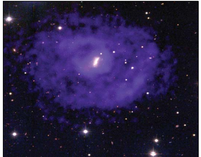
Figure 192: Dwarf Galaxy. An enormous hydrogen disk (blue) surrounds the dwarf galaxy UGC 5288 (bright white). This isolated galaxy, 16 million light-years from Earth, contains about 100,000 stars and is 1/25 the diameter of our Milky Way Galaxy, which has at least 100,000,000,000 stars. The dwarf’s mass is about 30 times too small to gravitationally hold onto the most distant hydrogen gas, so gravity could not have pulled the distant hydrogen gas into its disk. Because the gas is too evenly distributed and rotates so smoothly, it was not expelled from the galaxy or pulled out by a close encounter with another galaxy.
