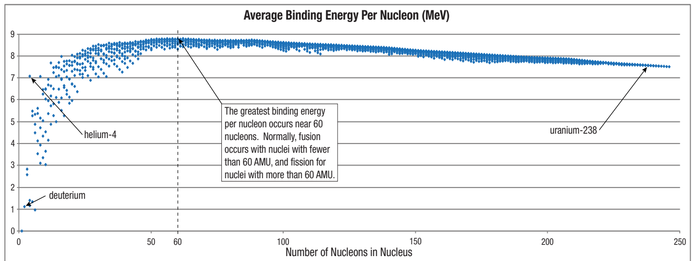
Figure 167: Binding Energy. When separate nucleons (protons and neutrons) come together to form a nucleus, a tiny percentage of their mass instantly disappears and becomes a large amount of energy. That energy (usually measured in units of Millions of electron Volts, or MeV) is called binding energy , because a powerful force—appropriately called the strong force —tightly binds the nucleons together—snaps them powerfully together—producing a burst of heat. Binding energy is also the energy required to unbind a nucleus or cluster of nucleons into their separate protons and neutrons.
