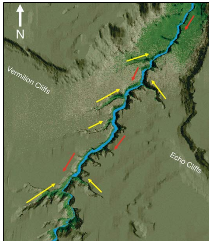
Figure 125: The Funnel and Barbed Canyons. This computer-generated picture resembles a photograph taken from 35,000 feet above the "barbed" side canyons feeding into the Colorado River. (The diagnostic importance of barbed canyons will soon be explained.) Flowing surface and subsurface water carved the barbed canyons in a direction (yellow arrows) opposite to the flow of the Colorado River today (red arrows). Notice that Echo Cliffs and Vermilion Cliffs nearly align. The funnel-shaped opening in the top right corner cut through a single cliff system, giving us these two sets of cliffs today. A giant, high-pressure hose, gushing from the upper right corner in the direction of the red arrows, would carve the funnel nicely.
