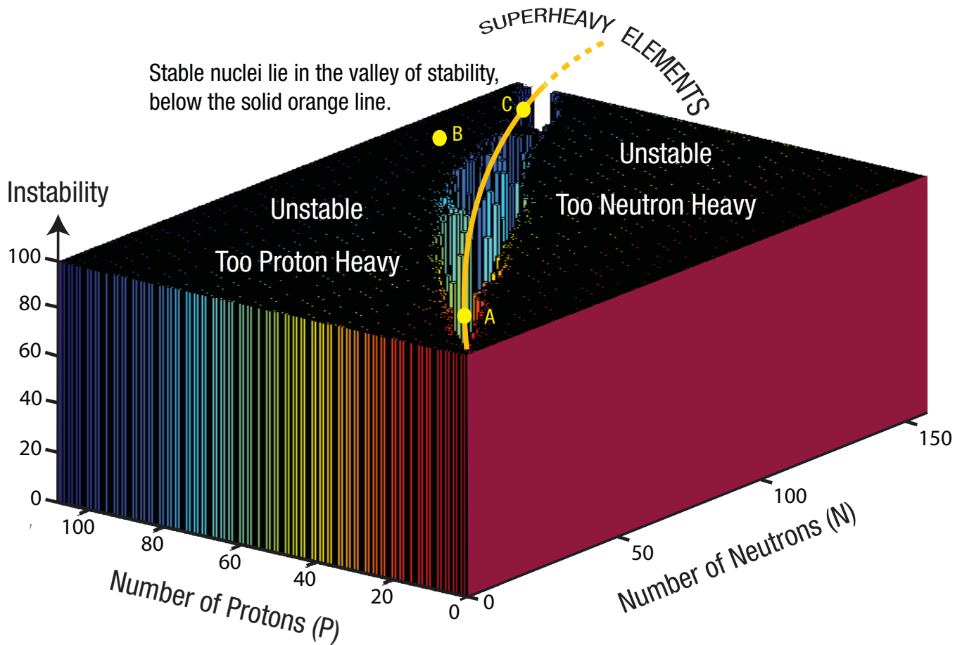
Figure 168: Valley of Stability. Each of the more than 3,100 known isotopes is defined by two numbers: the number of protons ( P ) and the number of neutrons ( N ). Think of each isotope as occupying a point on a horizontal P – N coordinate system. A thin, vertical bar represents each isotope's stability: tall bars for isotopes that decay rapidly, shorter bars for isotopes with longer half-lives, and no vertical bars for stable isotopes. 10 Almost 300 stable isotopes are represented far below the curved orange line, in what is called the valley of stability . It lies near the diagonal between the P axis and the N axis.
