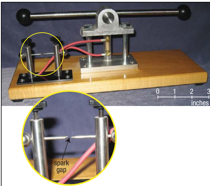
Figure 175: Piezoelectric Demonstration. When I rotate the horizontal bar of this device, a tiny piezoelectric crystal (quartz) is compressed in the vertical column just below the bar's pivot point. The red cables apply the generated voltage across the two vertical posts mounted on the black, nonconducting platform. Once the increasing voltage reaches about 4,000 volts, a spark (a plasma) jumps the gap shown in the circular inset. When the horizontal bar is rotated in the opposite direction, the stress on the quartz crystal reverses, so a spark jumps in the opposite direction.
